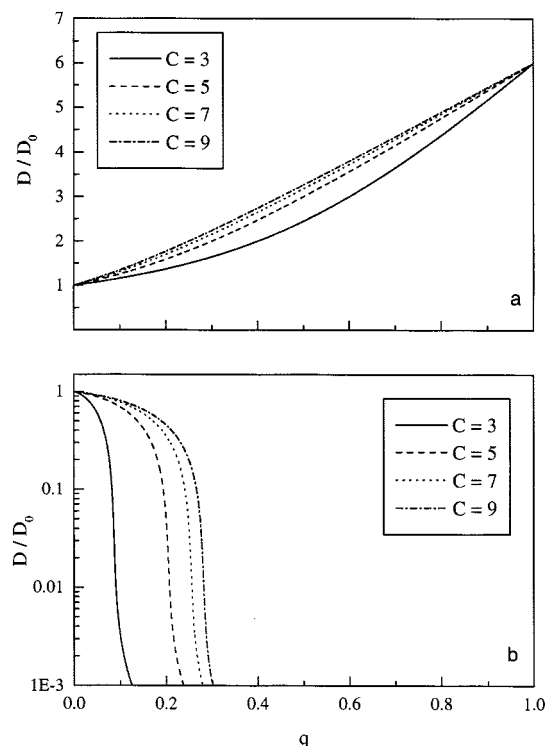
Figure 4. Theoretical dependencies of diffusivity on pore-filling ( q ) for various connectivity ( C ).
