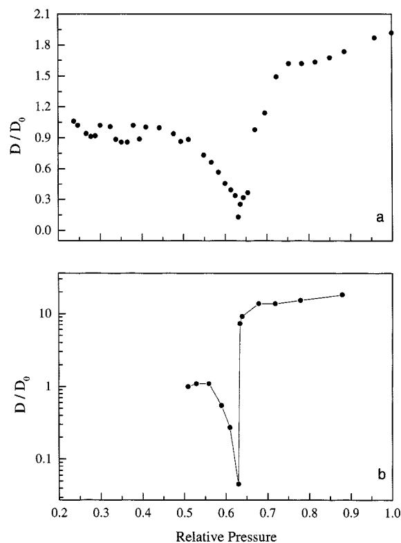
Figure 13. Experimental desorption diffusivity data.
